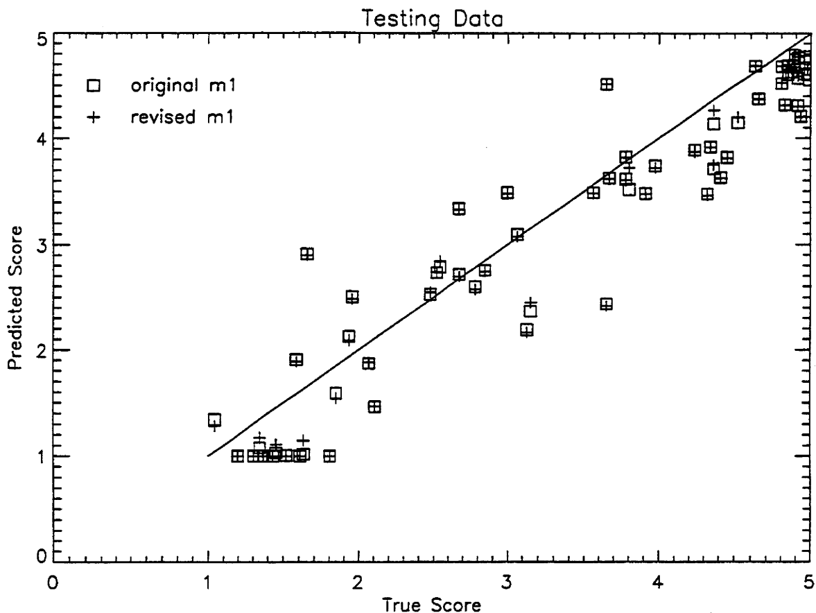
Figure 1 Prediction Performance, 64 Test Scenes
